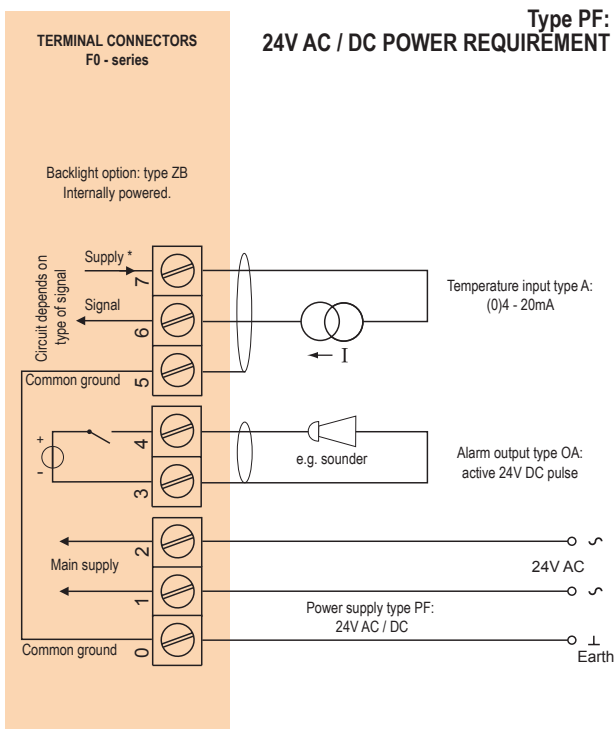
Typical wiring diagram Fo43-A-OA-PF-ZB
