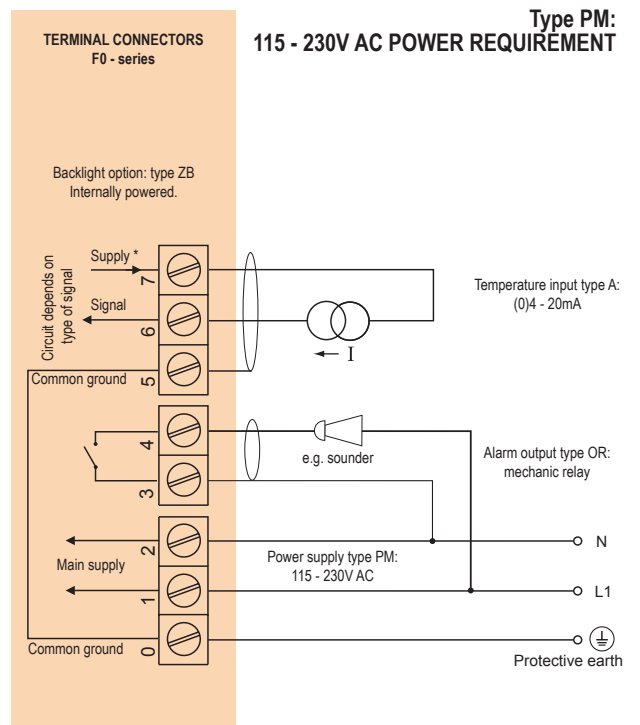
Typical wiring diagram Fo43-A-OR-PM-ZB
