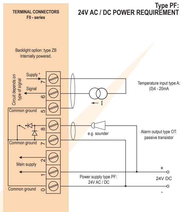
Typical wiring diagram Fo43-A-OT-PF-ZB
