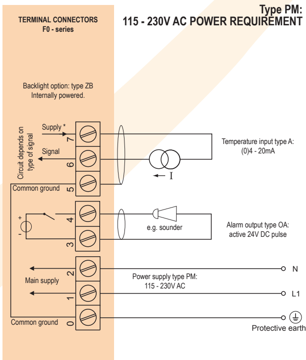
Typical wiring diagram Fo43-A-OA-PM-ZB
